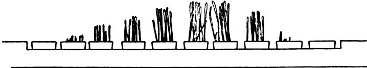
FIG. 110. — Effect of different temperatures upon Oats grown in a differential thermostat, an instrument evenly heated from the right side and cooled from the left; \times \frac{1}{4} . (Drawn from a photograph.)
